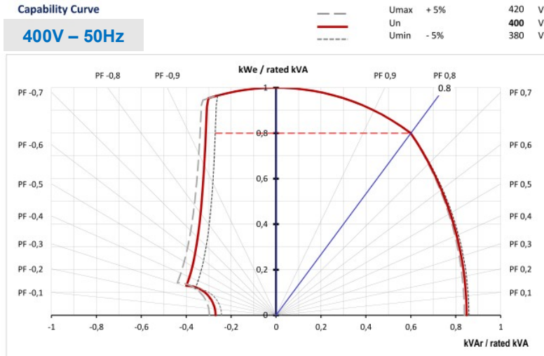
Capability Curve
